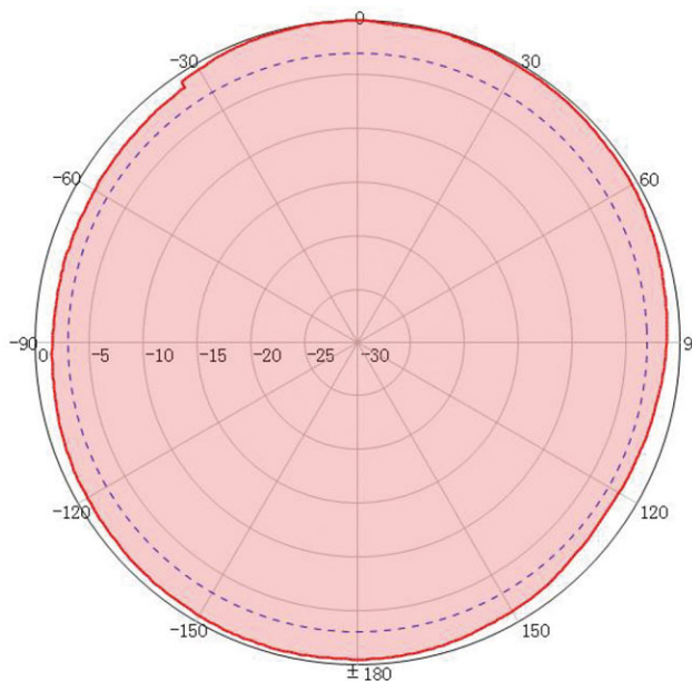
Axial Ratio
